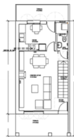
P. 30/4 Sup. Constr. = 41.45m² 1/2 Terr. = 4.89m² 46.34m²
